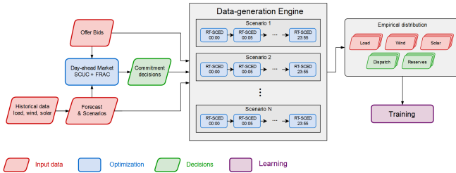
Fig. 5: Flow-chart of the Just-in-time Learning pipeline. Left: day-ahead market clearing. Middle: data generation using day-long simulations. Right: empirical distributions of load, wind, solar, and dispatch decisions are used as training data.
