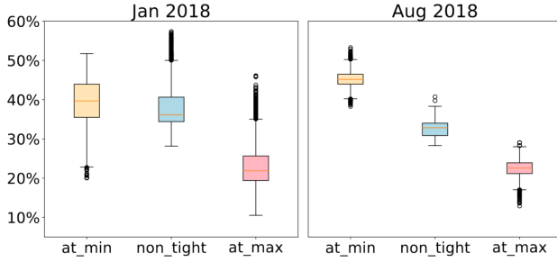
Fig. 3: Proportion of Generators at their Maximum and Minimum Limits in January (left) and August (right).
