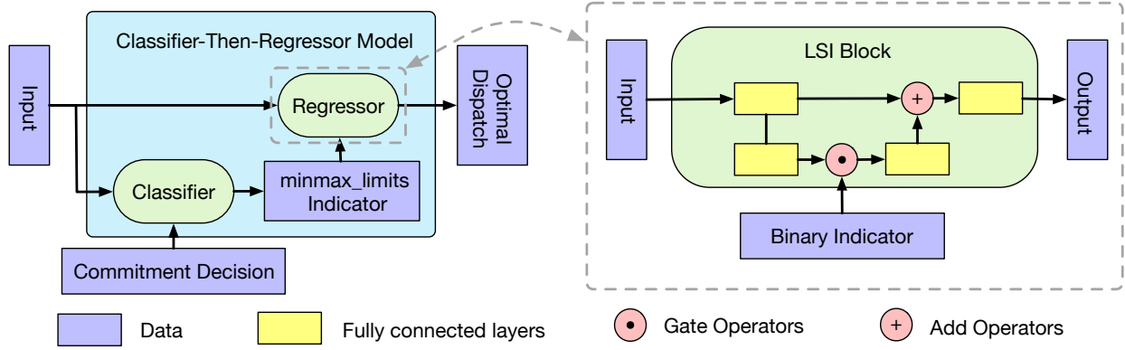
Fig. 4: The Proposed ML Model: 1) the figure on the left shows the structure of the Classifier-Then-Regressor model, where the outputs of the classifier are used to inform the subsequent regressor. Thus the regressor only needs to predict the dispatches of non-tight generators; 2) the figure on the right shows the structure of the regressor, i.e., a LSI block, where a gate operation takes the binary indicator to dropout some neurons of the previous fully connected layer.
